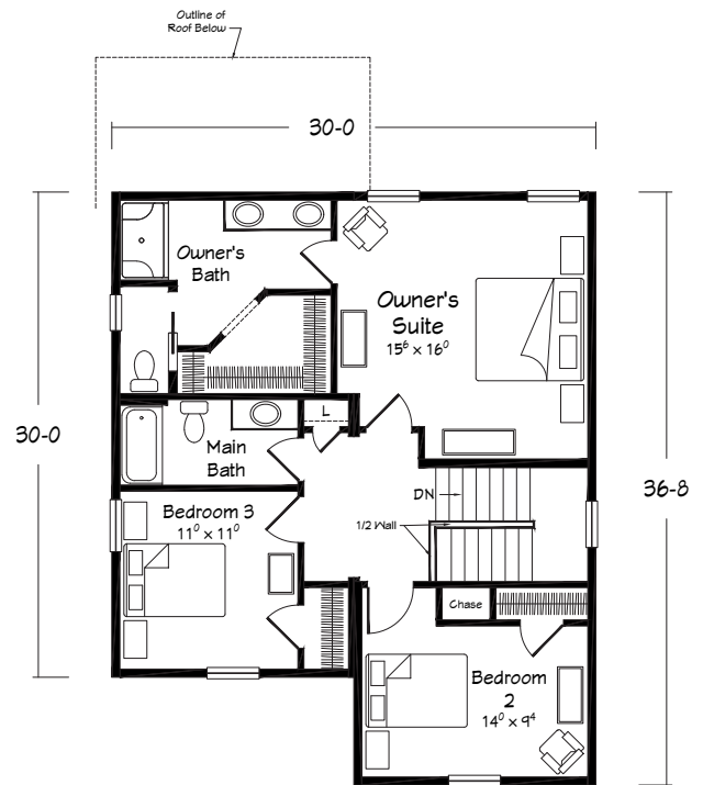
SECOND FLOOR LIVING 998 SQ. FT.
